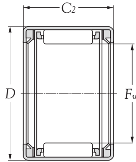
Type HK..LL (Open end. single seal)
