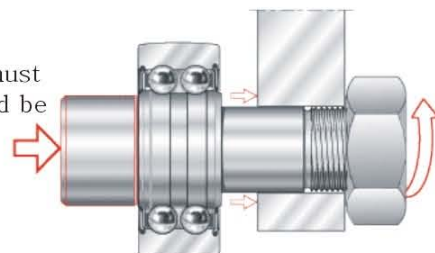
Fitting of a stud type track roller
