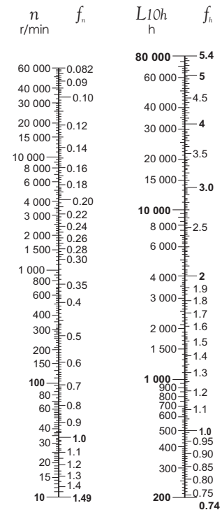
Fig. 4.1 Bearing life rating scale
